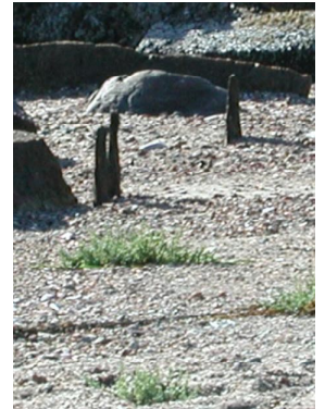
Pond-side sheathing, Bell Mill Edmunds ME is supported by sill timber.
